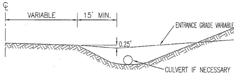
CUT SECTION
